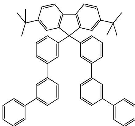
BuF(BS4) 2
