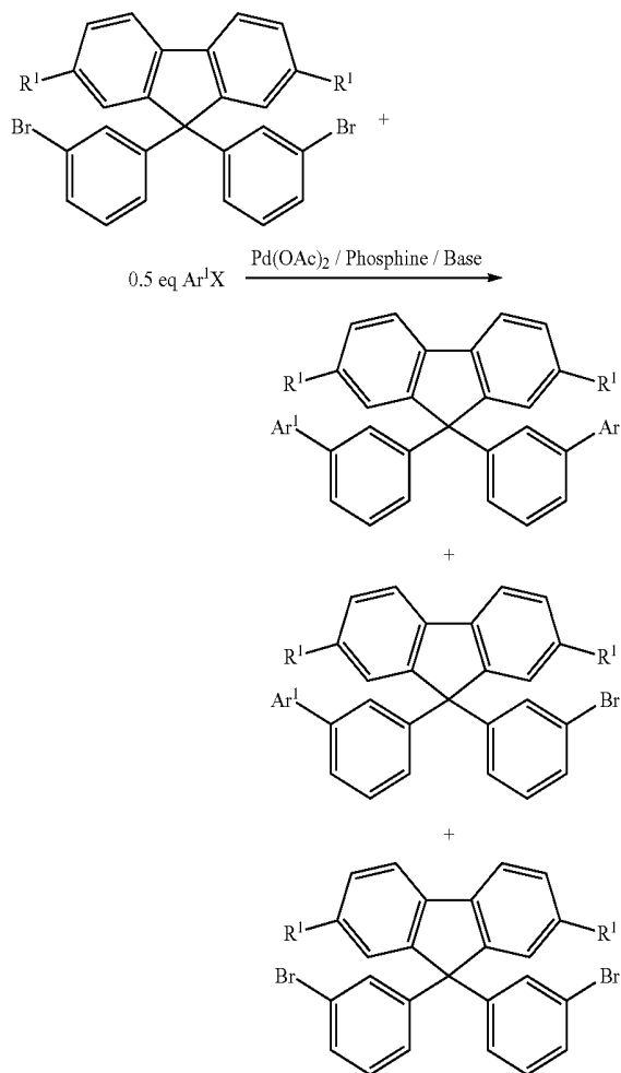
Scheme 4
