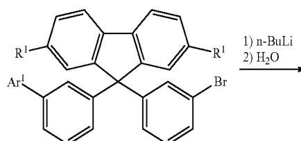
Scheme 5
