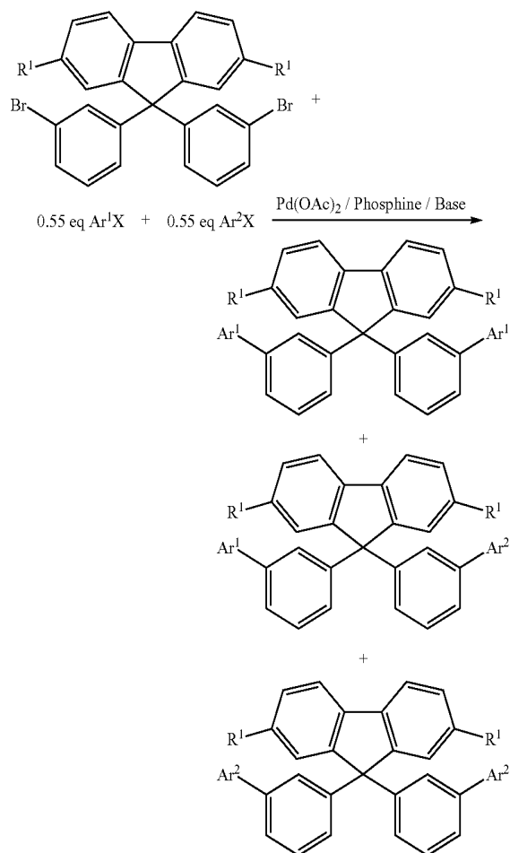
Scheme 3
